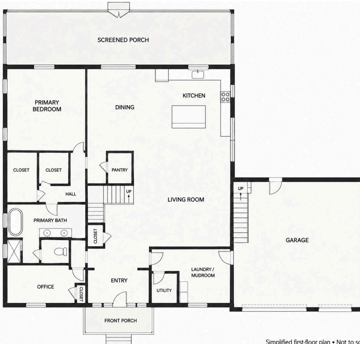
Simplified first-floor plan • Not to scale
